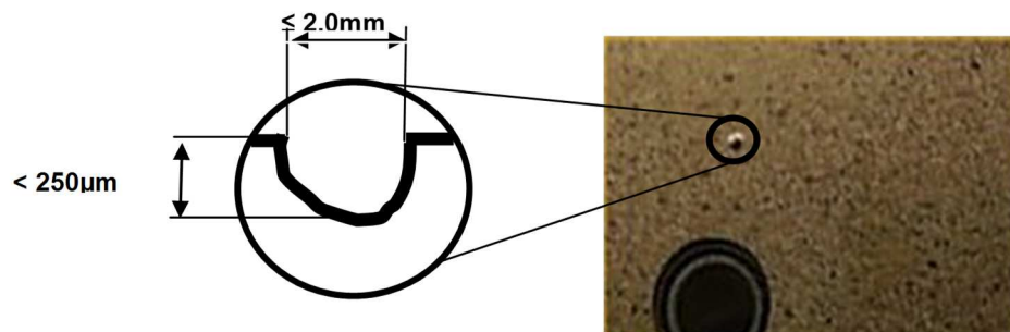
Figure 6: Etching hole (hole not down to substrate level) in the MiniSKiiP bottom surface
