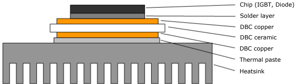
Figure 18: SKiM®4 sketch – cross section view
