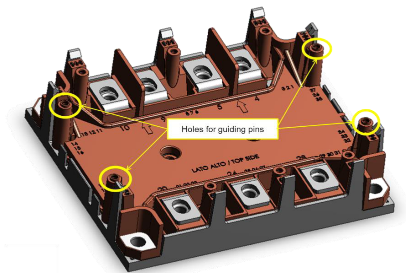
Figure 44: Guiding pin positions of SKiM®4
