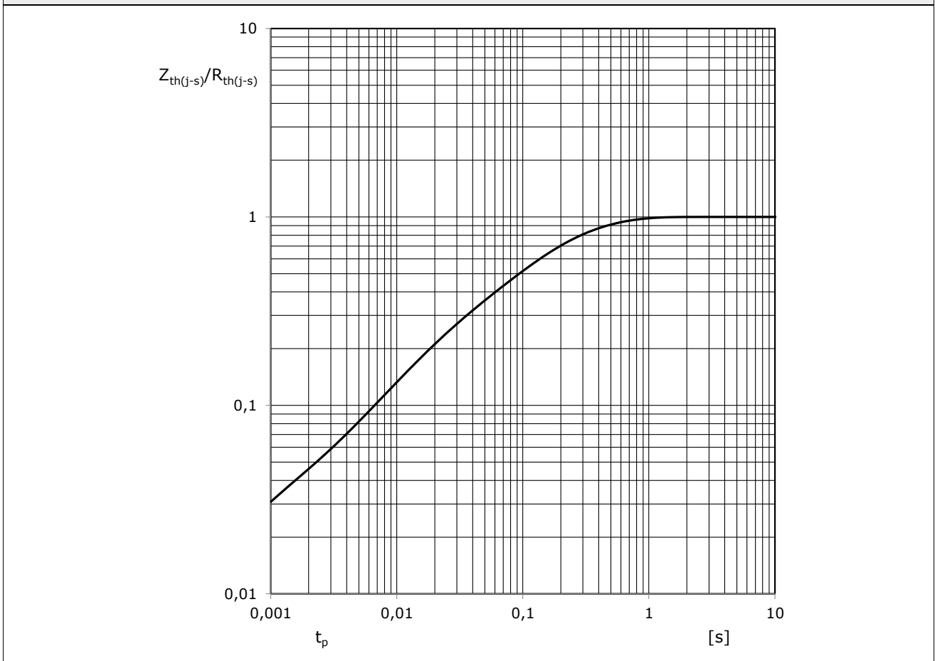
Figure 25: Standardized transient thermal impedance of SKiM®4 MLI and SKiM®4 TMLI
