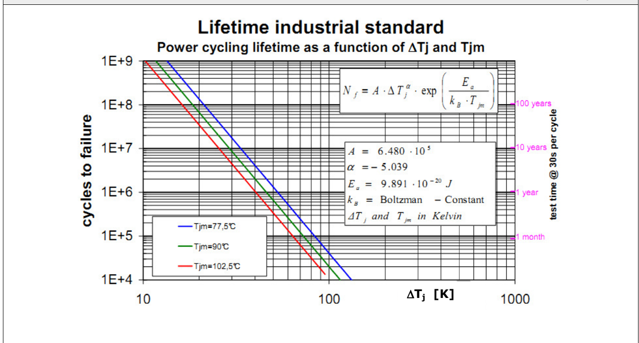
Figure 52: Power cycling value N_f as a function of the temperature cycling amplitude \Delta T_j
