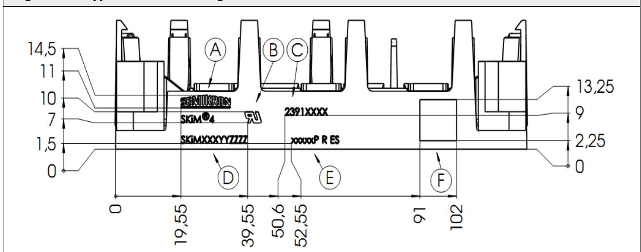
Figure 53: Typical laser marking of SKiM®4
