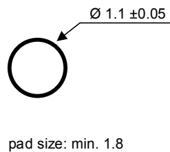
Figure 21: SKYPER® 32 2nd edition | Finished hole & pad size in mm
