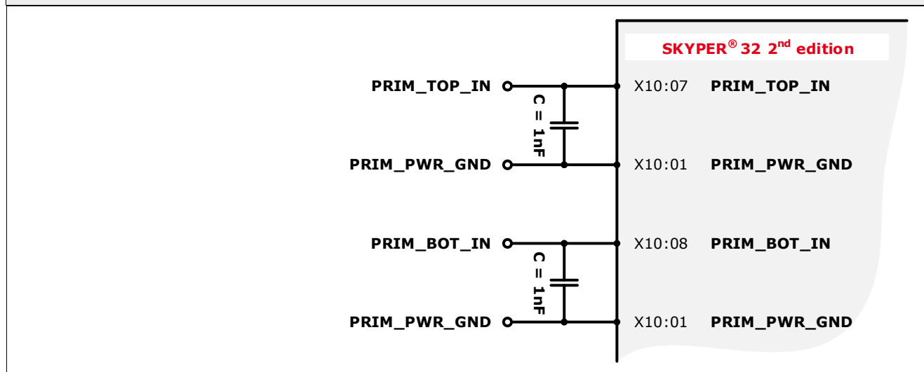
Figure 8: SKYPER® 32 2 nd edition | TOP / BOT input
