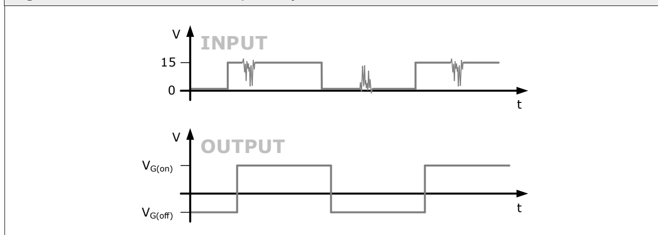
Figure 9: SKYPER® 32 2 nd edition | Pulse pattern – SPS
