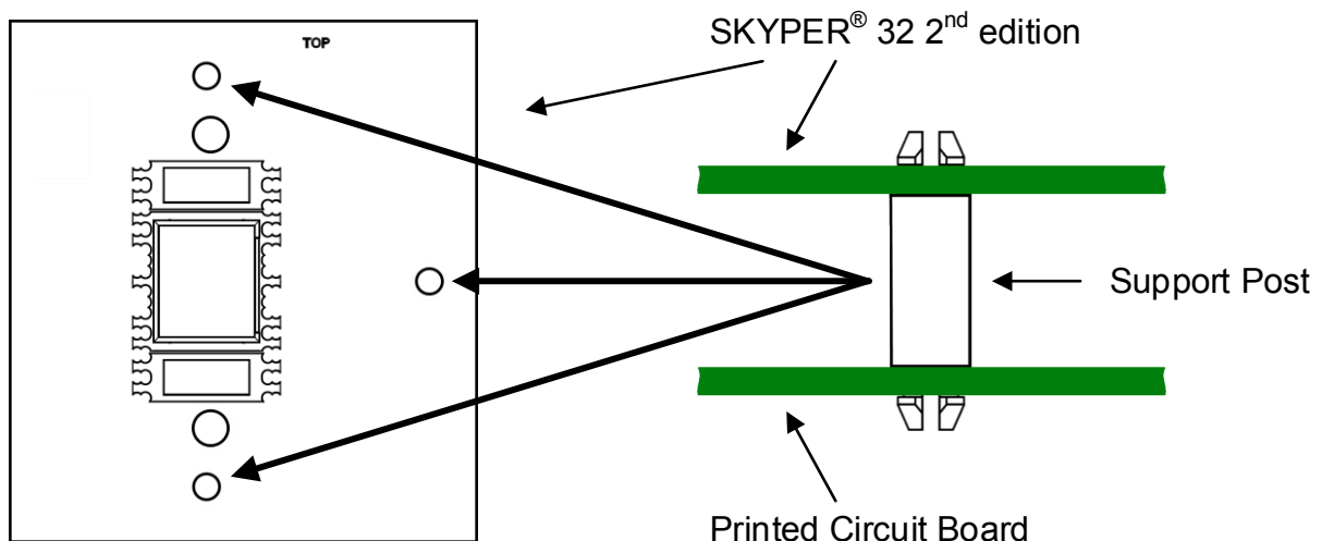
Figure 22: SKYPER® 32 2nd edition | Use of support posts
