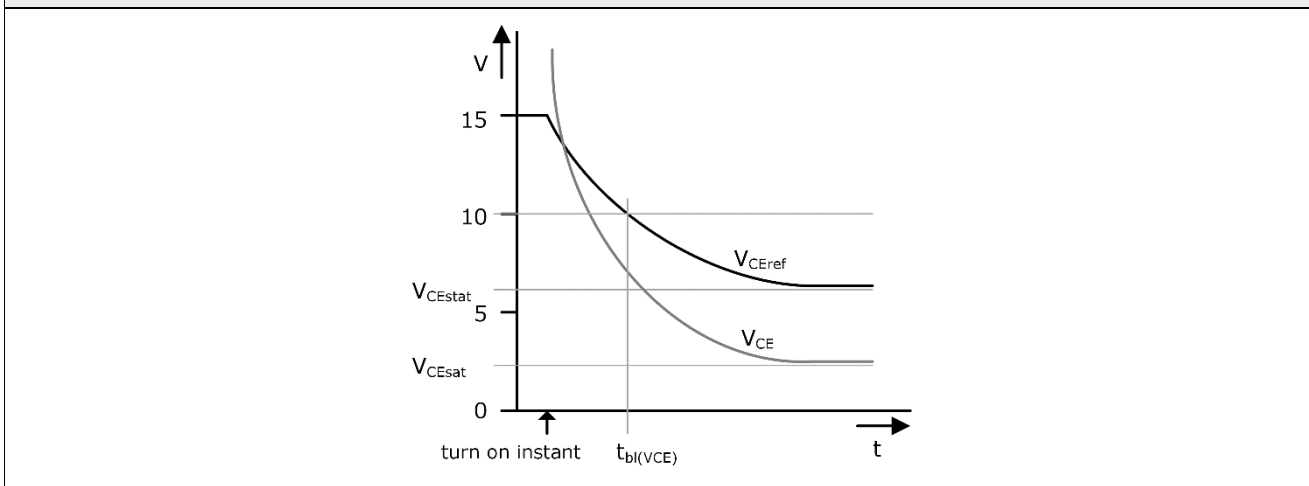
Figure 5: SKYPER® 12 PF | Reference voltage ( V_{CEref} ) characteristic
