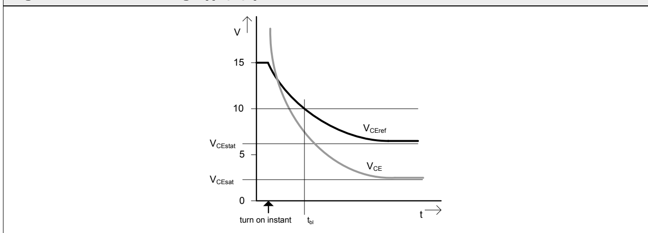
Figure 6: Reference Voltage ( V_{CEref} ) Characteristic
