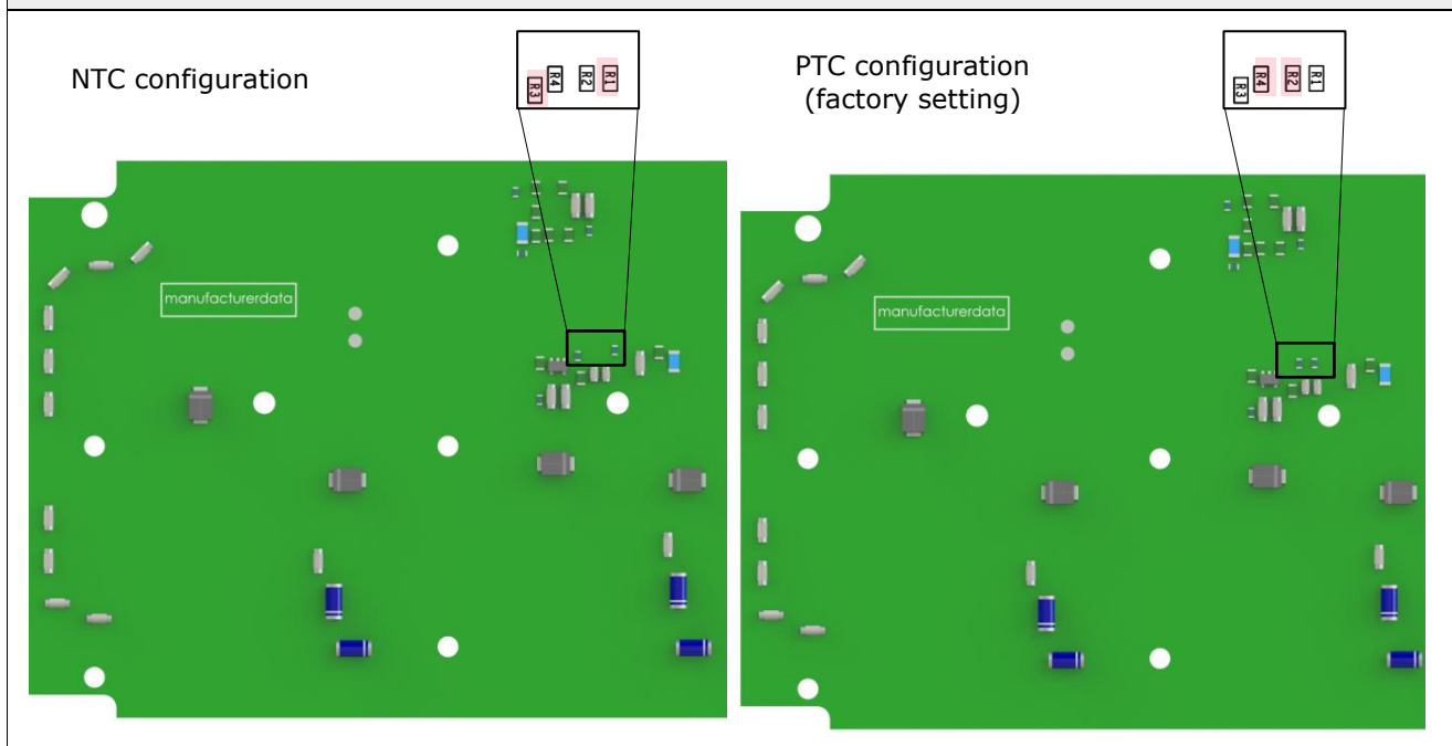
Figure 5: Over temperature protection configuration of NTC and PTC temperature sensor versions (BOT View)
