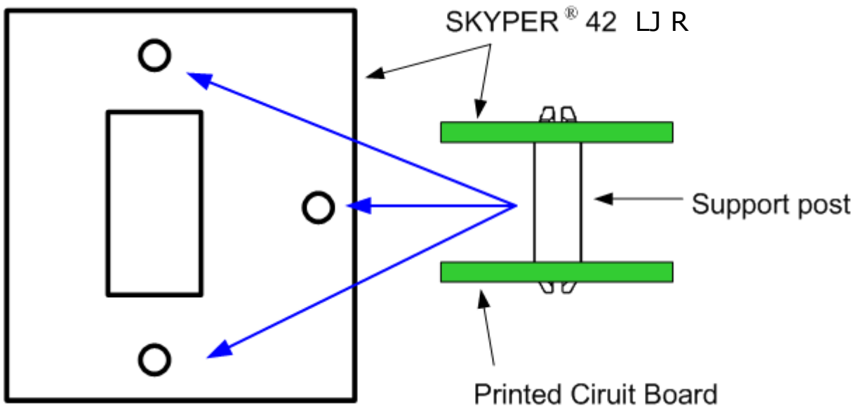
Figure 9: Driver Core Mounting
