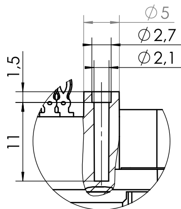
A (2 : 1) Cut-out shows section through the center of PCB-dome
