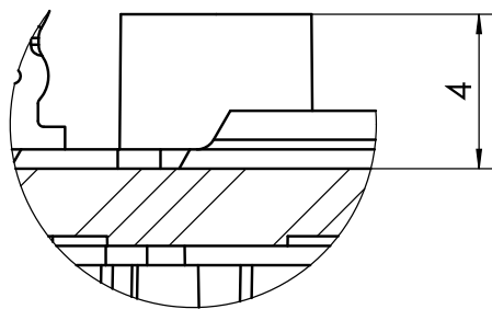
B (5 : 1) Sectional plane in the middle of module
