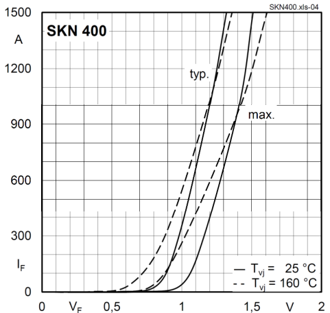
Fig. 5 Forward characteristics
