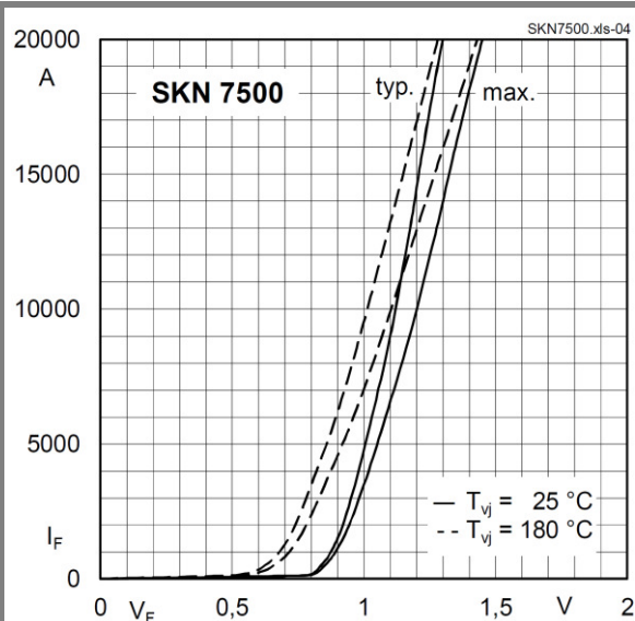
Fig. 4 Forward characteristics
