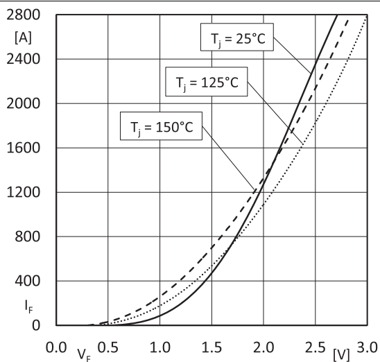
Fig. 7: Forward charact. Diode (typical); I_F = f(V_F) ; (chiplevel)
