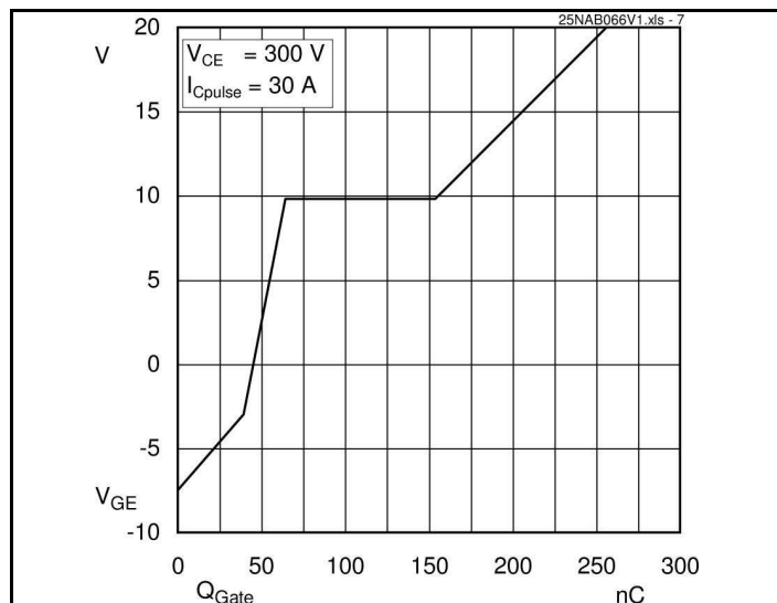
Fig. 7 Typ. gate charge
