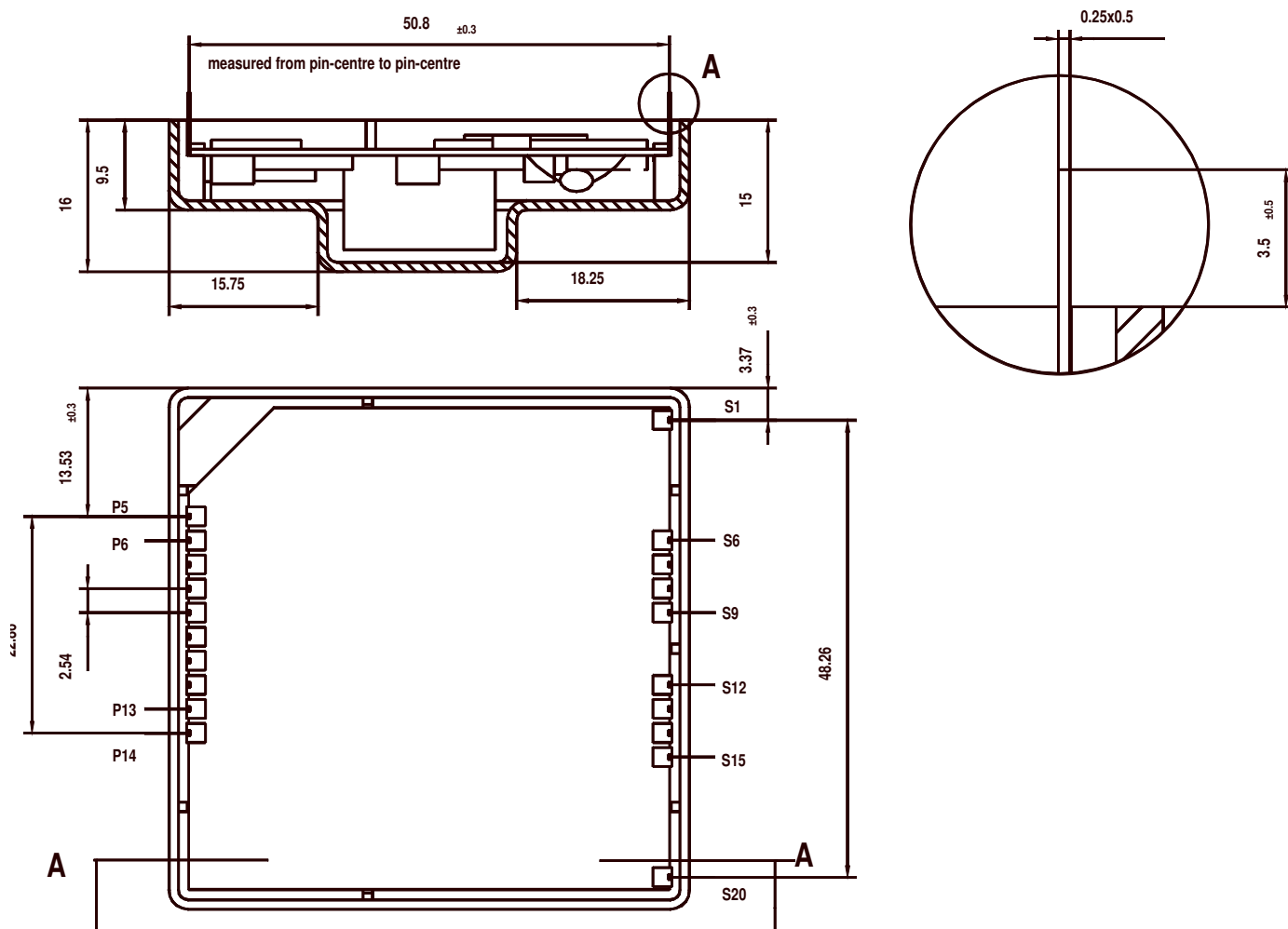
Fig. 2 Dimension drawing and PIN array (P5 and P6 are not existing for SKHI22A/21A)
