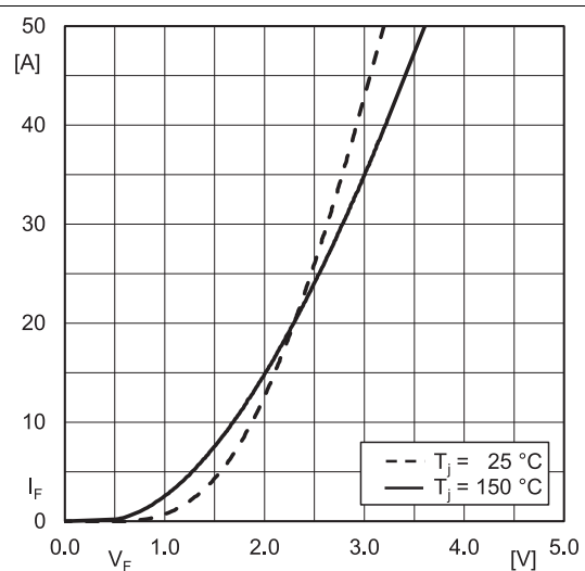
Fig. 10: Typ. Inv. diode forward charact., incl. R_{GG} + EE'
